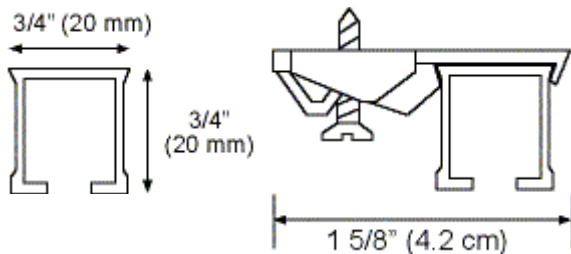
Track cross section with #SKS-3003-25 Ceiling Bracket smart click
